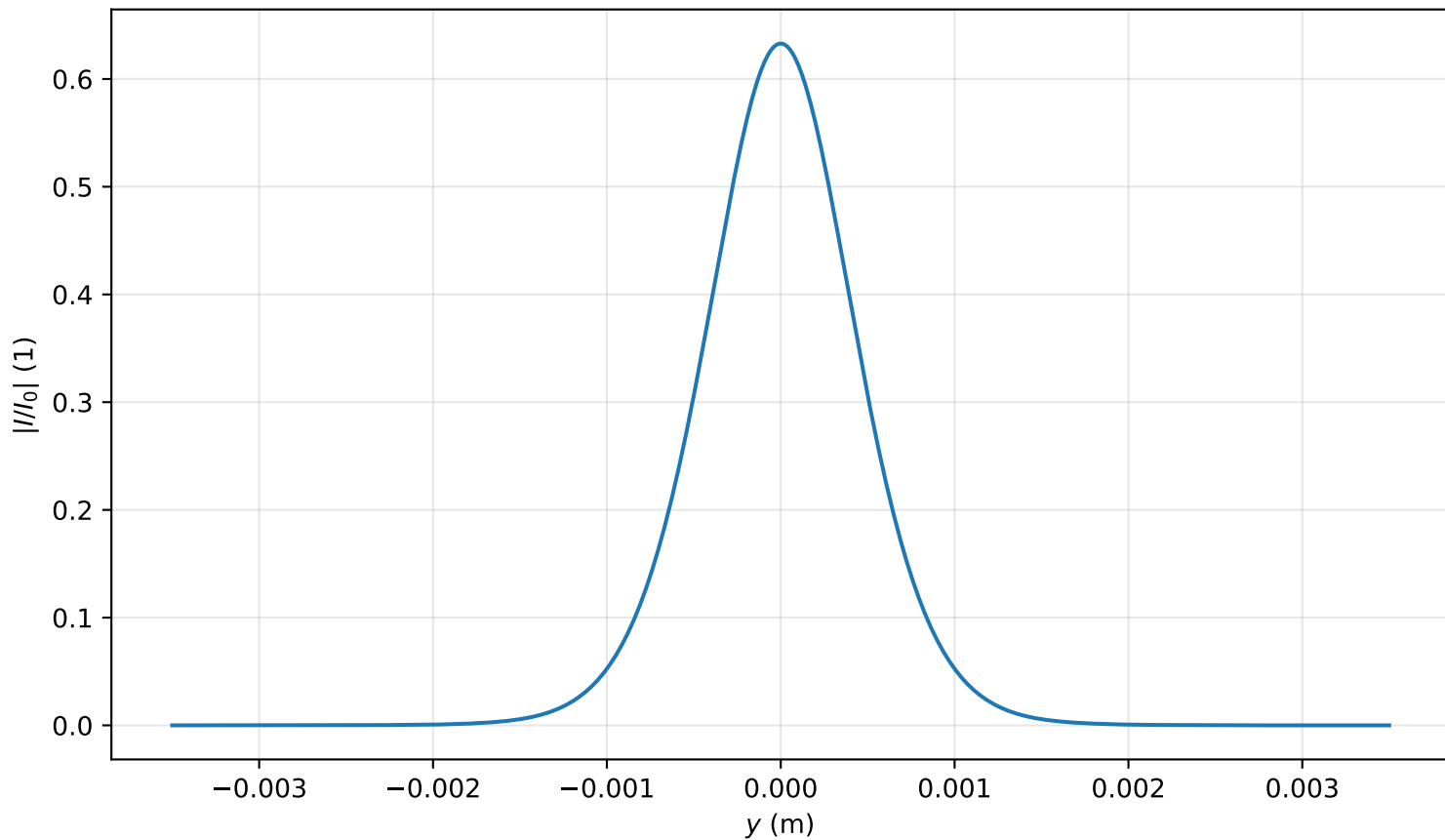
Intensity profile I(x=0, y, z=2.707)/I_0 , P_{in}=0.5P_{cr} , artificial time
